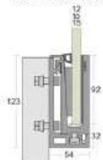
SG 28 CPS Side Mount Continuous Base Profile
