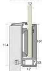
SG 09 BRCVS Brackets with Continuous Cover Profile
