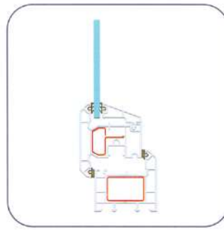
Casement Window
