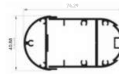
WSL01 tapered leg 75/45 x 40 mm
