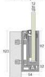
SG 28 BRS Brackets System
