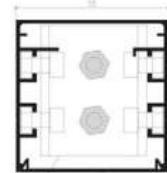
WSLQ55 Square leg 55 x 55 mm
